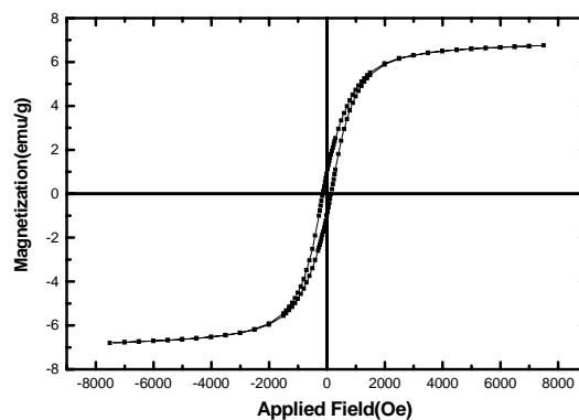
Fig. 5. Room temperature magnetization curves of (a) Fe 3 O 4 nanoparticles (b) CA/Fe 3 O 4 (10%) nanocomposite.
