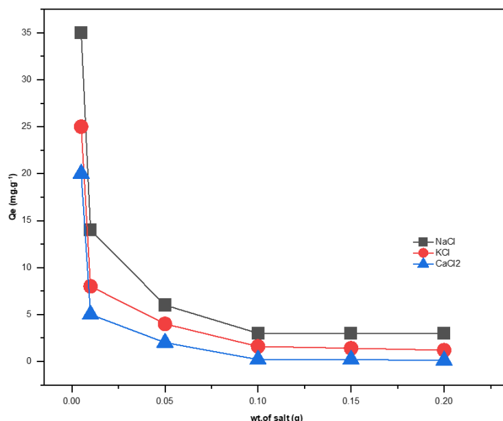
Fig. 12. Effect of ionic strength on the MTX adsorption.
