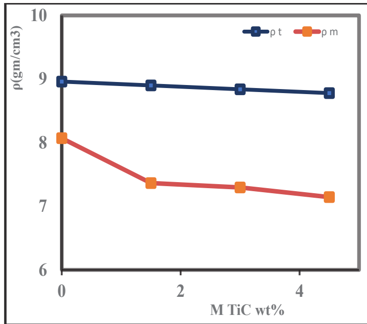
Fig. 11. Theoretical and measured densities for sintered Cu - micro size TiC composites.
