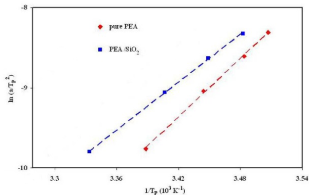
Fig. 14. Crystallization activation energies of selected samples
