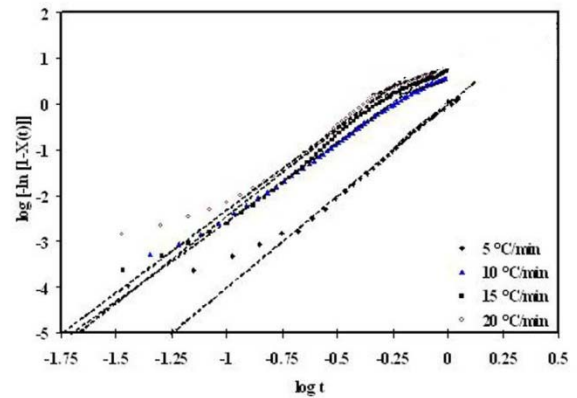
Fig. 9. Avrami curves of pure PEAd during non-isothermal crystallization
