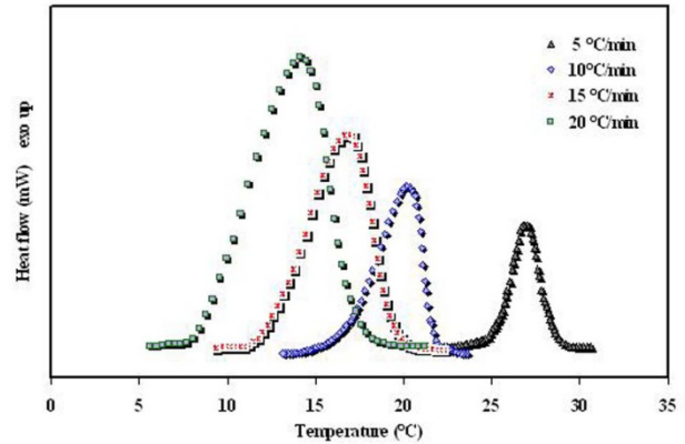
Fig. 4. DSC thermograms of non-isothermal crystallization for PEAd/SiO 2 3%wt. nanocomposite at different cooling rates.
