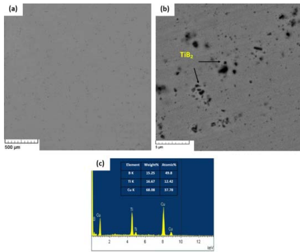
Fig. 1. a) Scanning electron micrograph of TiB 2 particles in copper matrix (b) shape and distribution of TiB 2 particles (c) EDX analysis of TiB 2 particles
