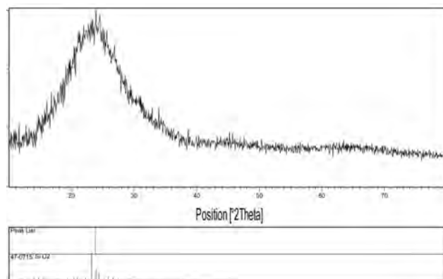
Fig. 3. XRD pattern of SiO 2 nanoparticles
