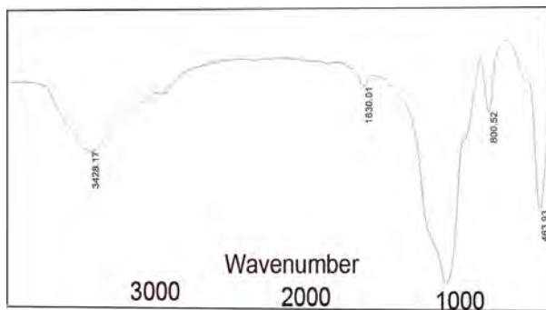
Fig. 8. FTIR spectrum of SiO 2 nanoparticles
