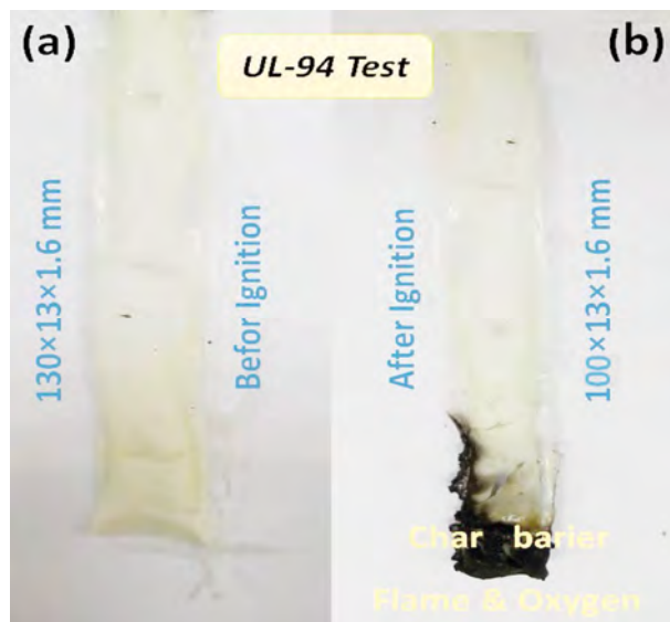
Fig. 9. UL94 of pure PS (a) before (b) after ignition
