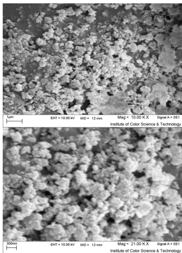
Fig. 6. SEM images of \text{SiO}_2 obtained by succinic acid
