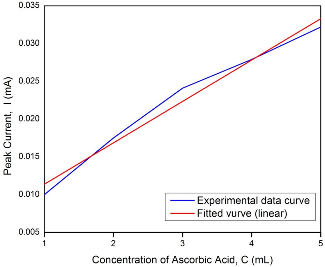
Figure S1 Trend line indicating the relationship between Peak Current I and Concentration C
