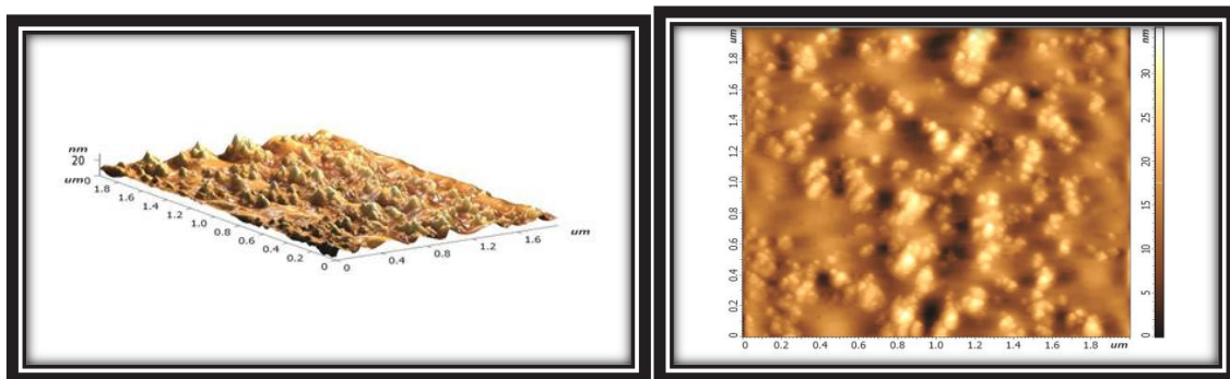
Fig. 3. AFM images: 3-Dimensional, 2-Dimensional \text{Fe}_3\text{O}_4 NPs.
