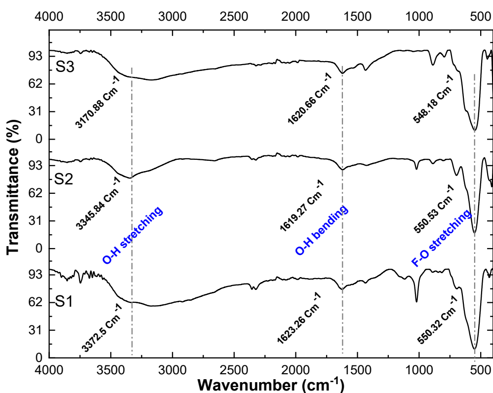
Fig. 2. FTIR spectra of Fe 3 O 4 MNP samples S1, S2, and S3, highlighting the main absorption regions of stretching and bending vibrations.
