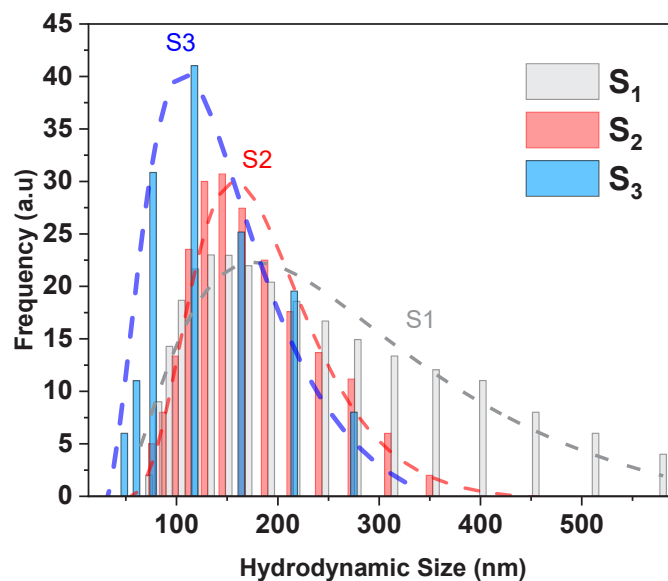
Fig. 4. DLS particle size distributions for Fe 3 O 4 MNP samples (grey), (red), and (blue). A log-normal function was used to fit the size distributions of the three samples.
