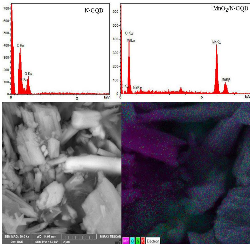
Fig. 3. EDX analysis of N-GQD and MnO 2 /N-GQD (top), SEM and mapping image of MnO 2 /N-GQD (bottom).
