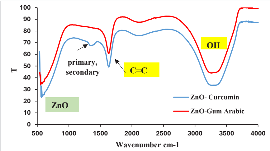
Fig.6. FTIR of ZnO colloidal.
