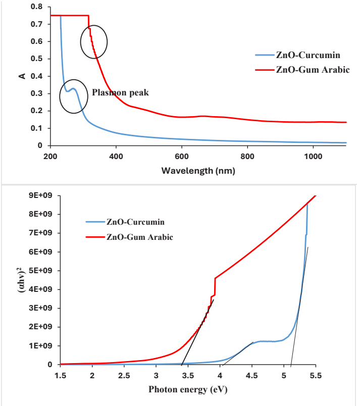
Fig. 7. Optical properties of ZnO colloidal.
