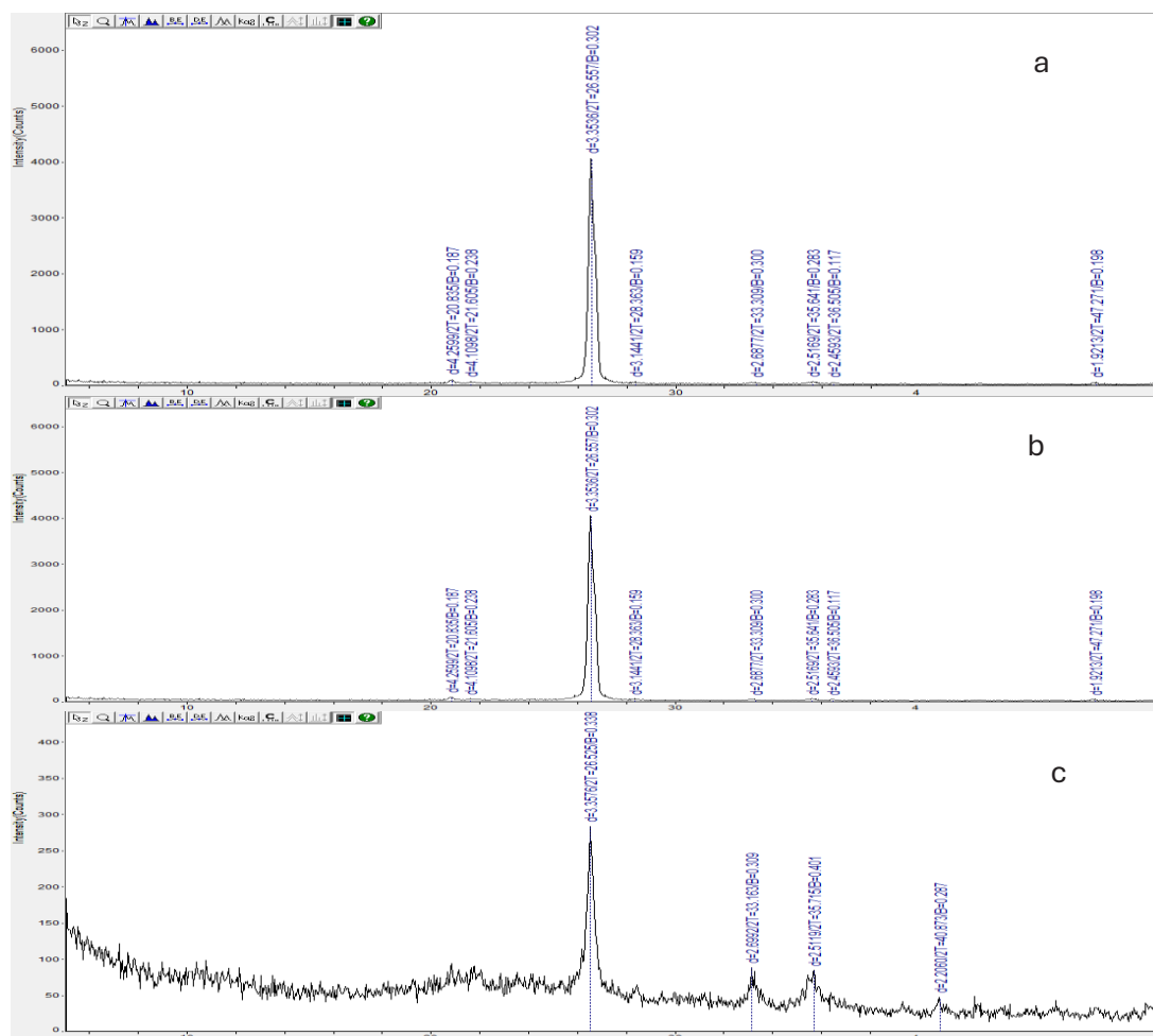
Fig. 4. XRD pattern of graphite (a), treated graphite with nickel sulfate (b), and purified nanographite (c).
