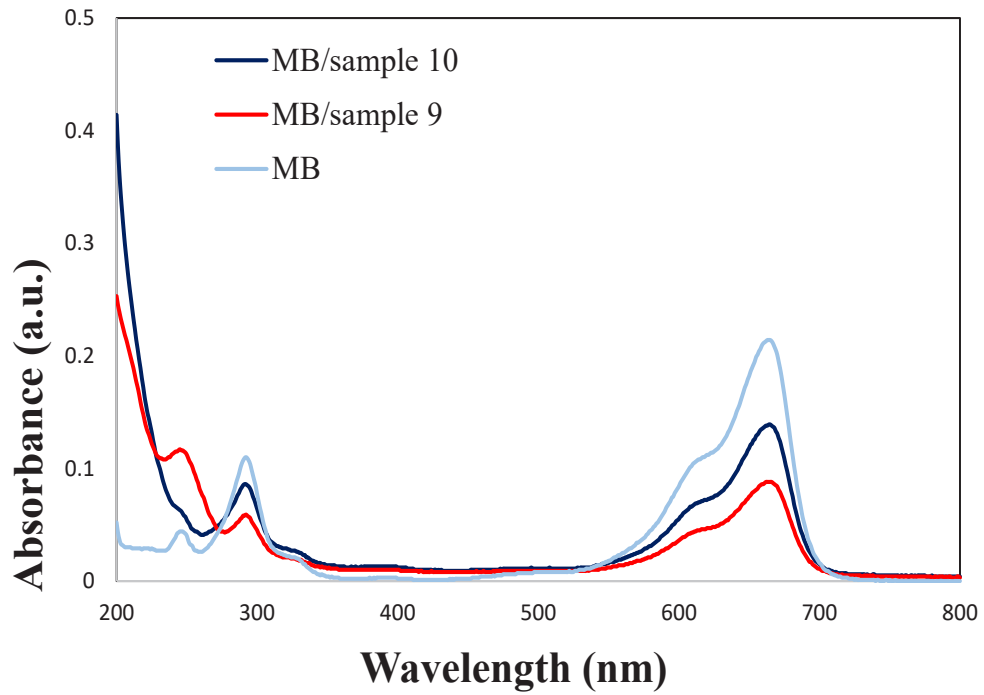
Fig. 8. Absorption spectra of MB and the solutions obtained from centrifugation of MB/samples 9 and 10 suspensions.
