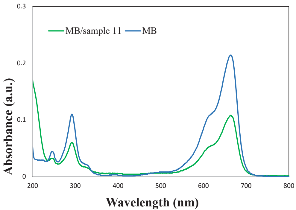
Fig. 9. Absorption spectra of MB and the solution obtained from centrifugation of MB/sample 11 suspension.
