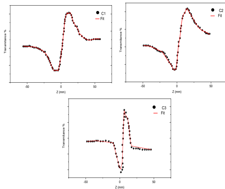
Fig. 11: Close aperture Z-Scan for 3 concentrations of ZnO NPs in distilled water using (200mW, 655nm).
