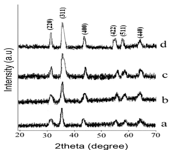
Fig. 1. XRD patterns of Ni_{1-x}Zn_xFe_2O_4 nanoparticles for a) x=0 , b) x=0.3 , c) x=0.7 and d) x=1 .
