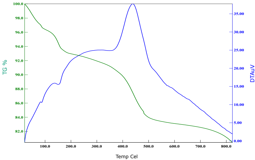
Fig .5 TG–DTA curves of the ZnO NPs
